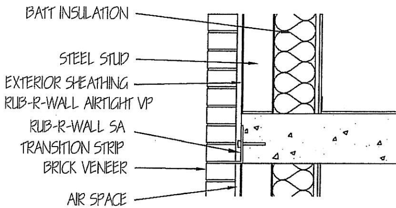
INTERMEDIATE FLOOR
