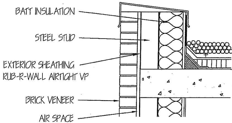
ROOF AT PARAPET WALL
