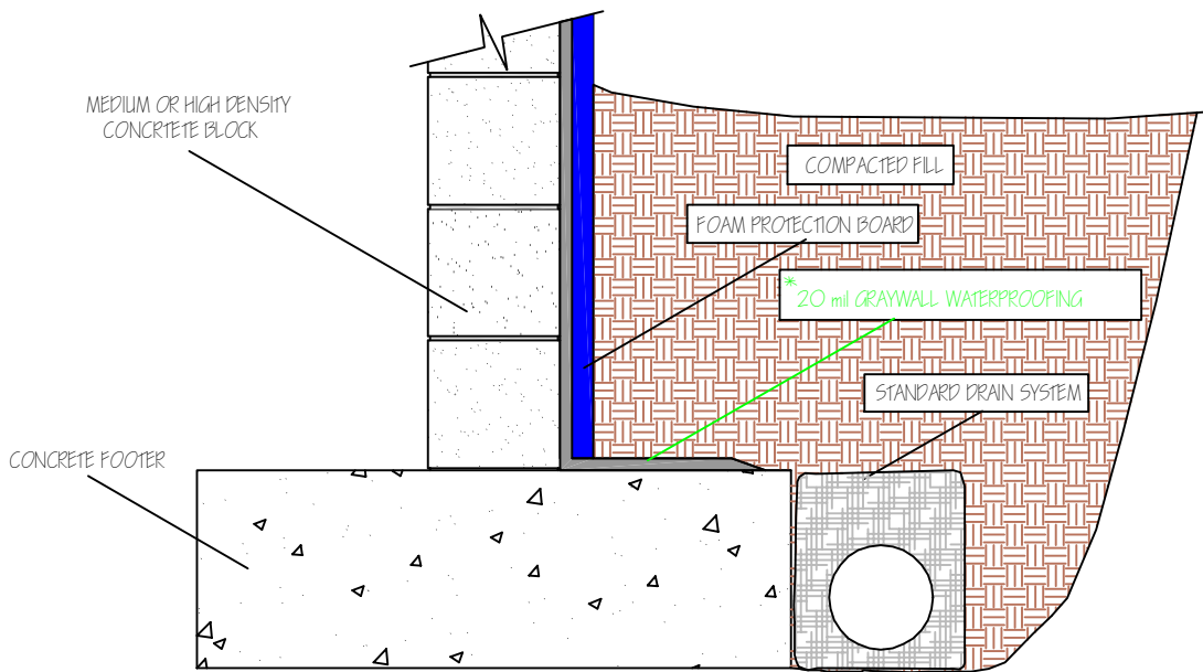
FIGURE NO 5A CONCRETE BLOCK WALL
