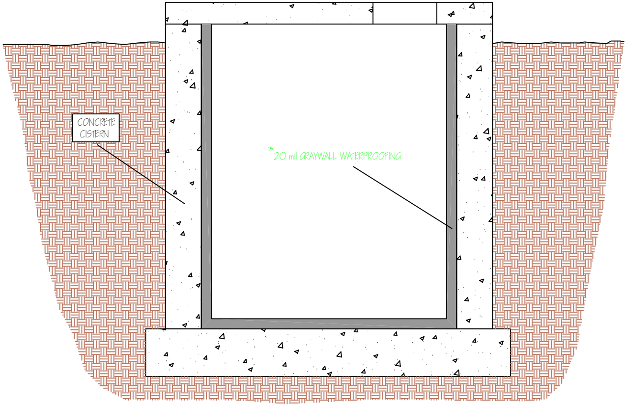
FIGURE NO 11 CONCRETE CISTERN WITH GRAYWALL F LINER
