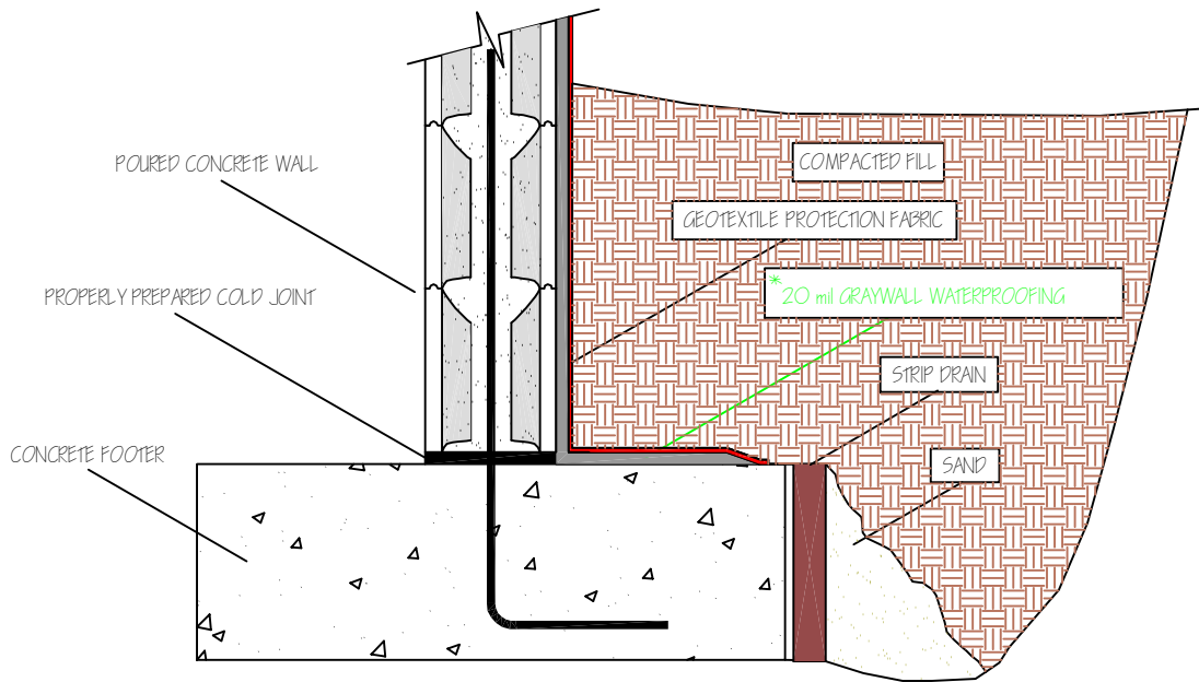
FIGURE NO 9 EPS FOAM FORM/ CONCRETE WALL
