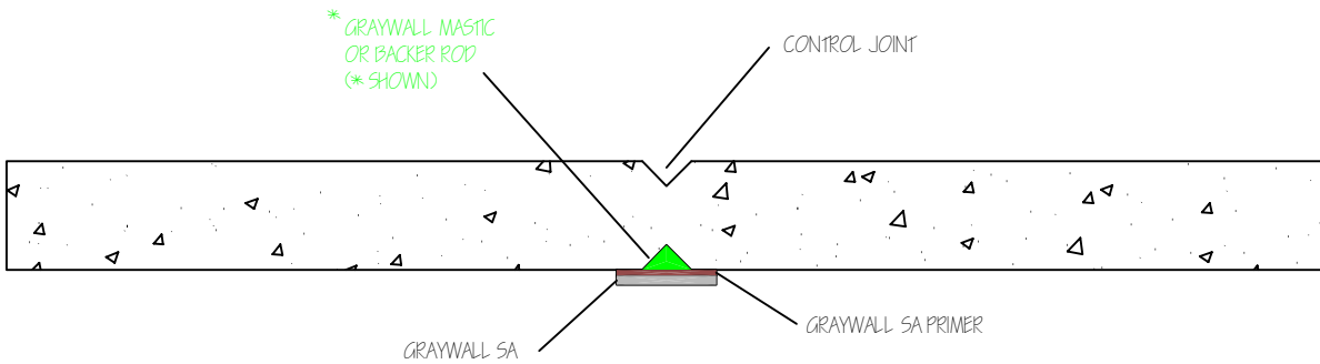
FIGURE NO 10 POURED CONCRETE WALL W/ CONTROL JOINT
