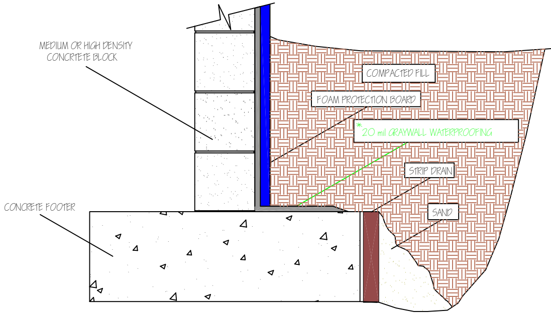
FIGURE NO 5 CONCRETE BLOCK WALL
