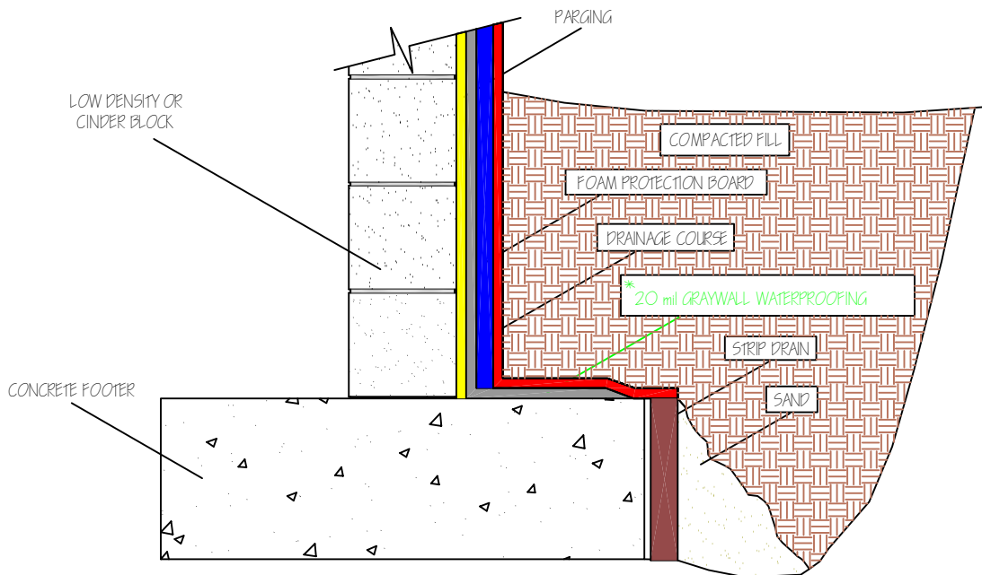
FIGURE NO 6 PARGED, LOW DENSITY BLOCK
