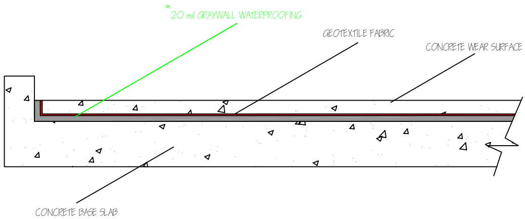
FIGURE NO 4 CONCRETE SUB-SLAB WITH CONCRETE WEAR SURFACE
