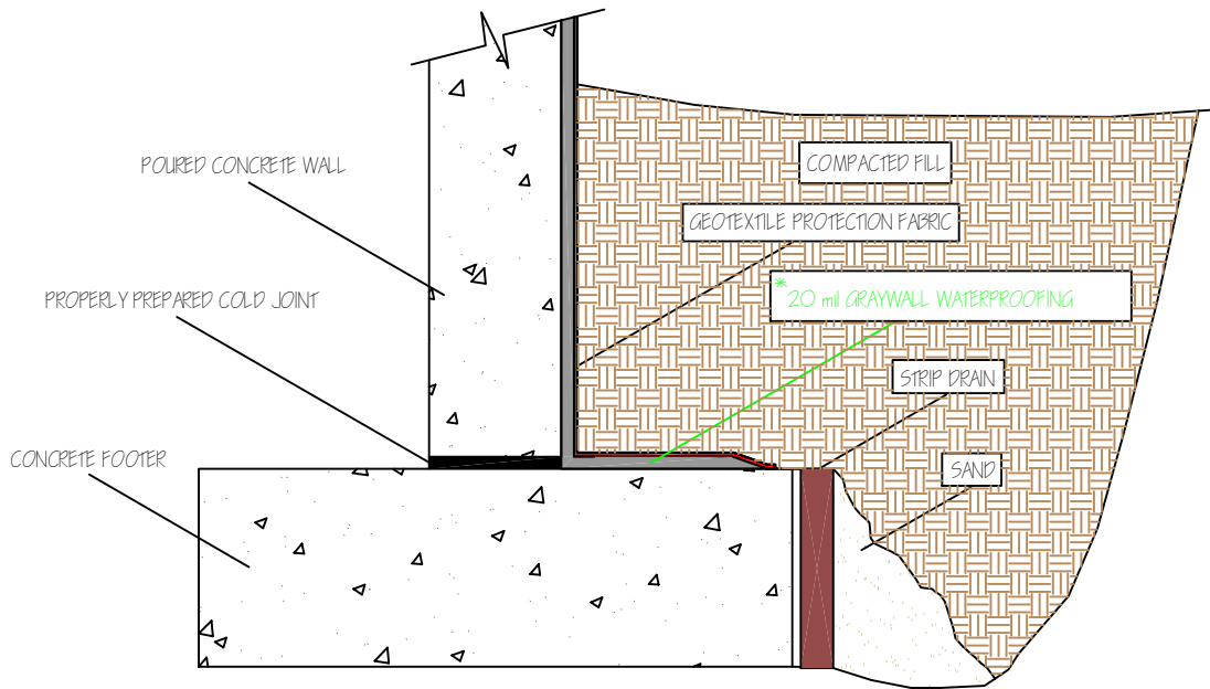
FIGURE NO 3 POURED CONCRETE WALL WITH STRIP DRAIN AND GEOTEXTILE PROTECTION SHEET
