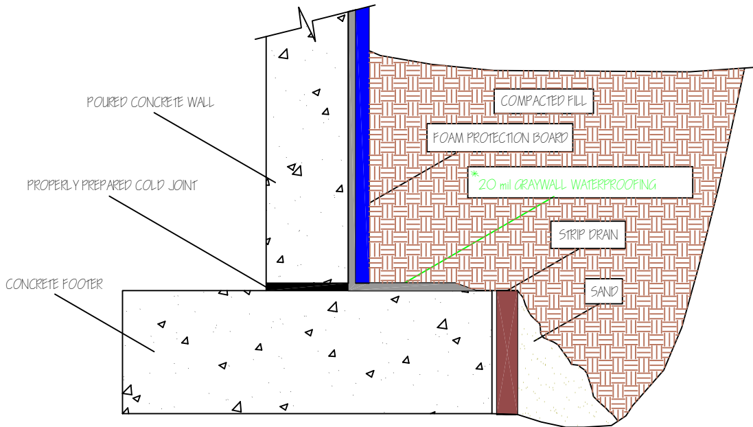
FIGURE NO 2 POURED CONCRETE WALL WITH STRIP DRAIN
