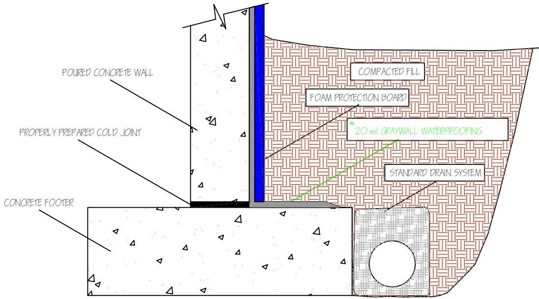
FIGURE NO 1 POURED CONCRETE WALL
